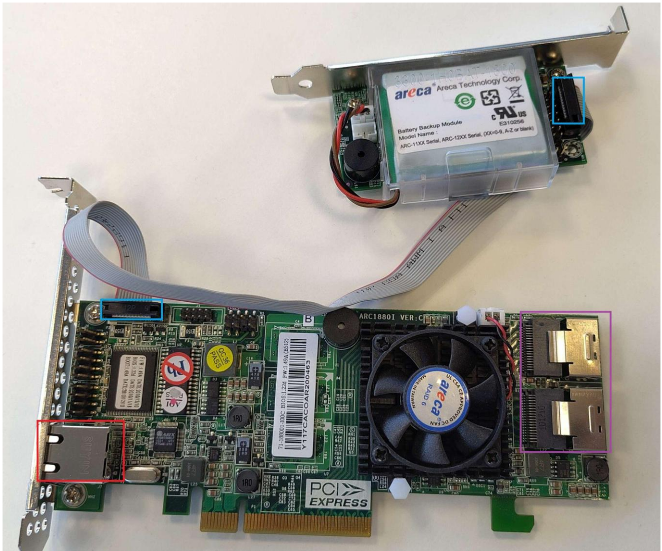
RAID controller card with backup battery module
